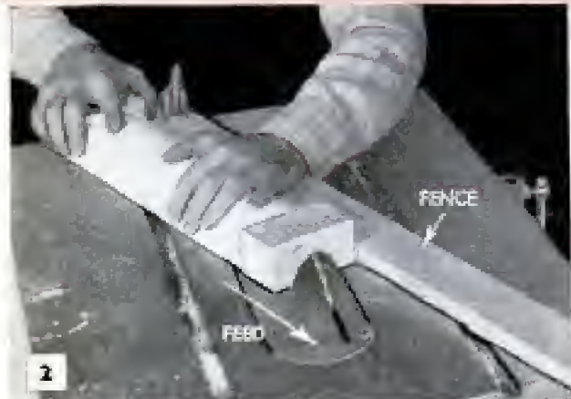
It is practical to use a saw blade for cove cuts up to about 45 deg., as above. The cuts are about 1/8 in. deep per pass. Below, the molding head is a true cutter and will cut any angle up to 90 deg. With it, cuts can be as deep as 1/2 in. per pass. The molding head performs better, but the saw can be very useful
